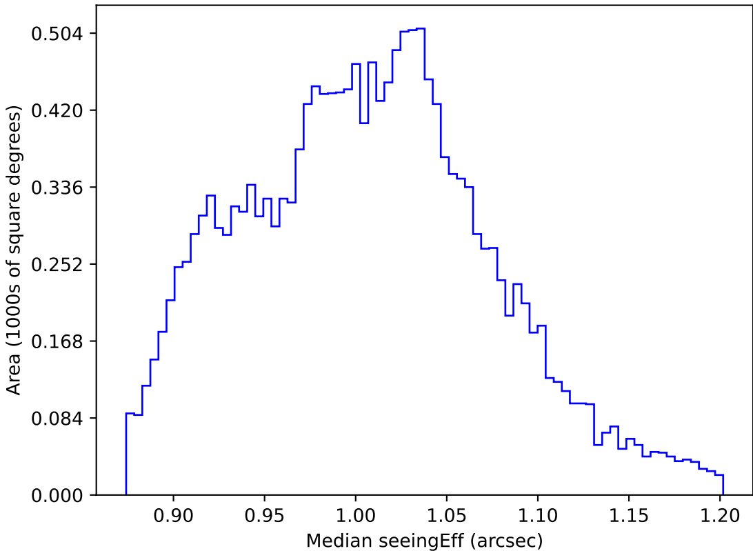
too_elab_r64_d2_gz_v3.4_10yrs WFD z band: Median seeingEff
