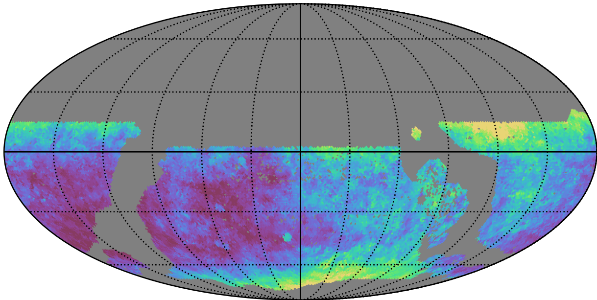
too_elab_r64_d2_gz_v3.4_10yrs WFD y band: Median seeingEff
