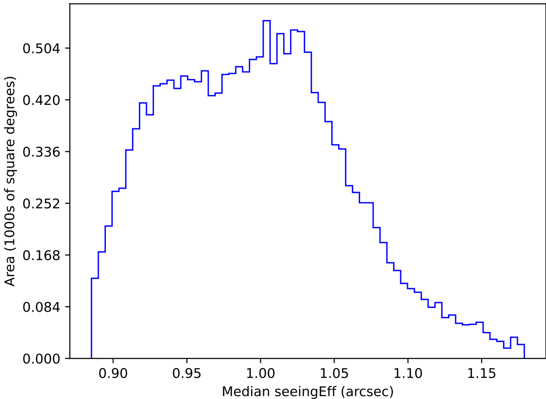
too_elab_r64_d2_gz_v3.4_10yrs WFD y band: Median seeingEff
