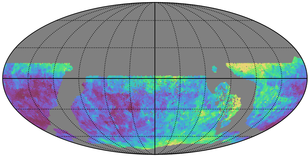
too_elab_r64_d2_gz_v3.4_10yrs WFD u band: Median seeingEff
