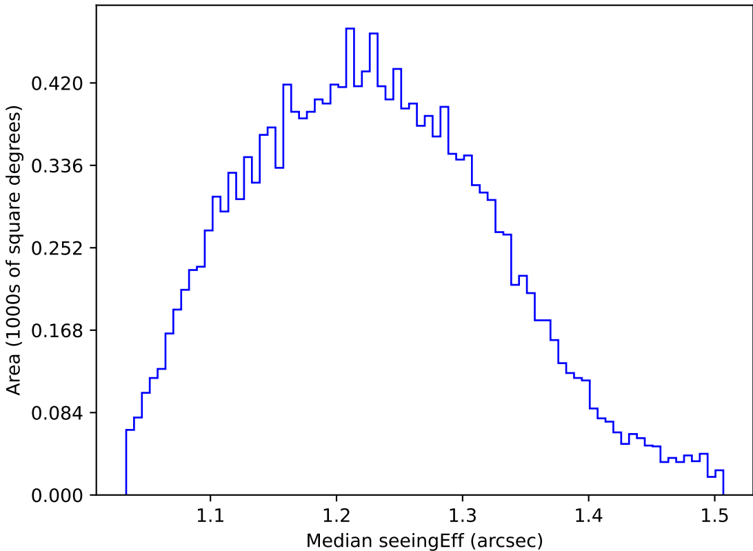
too_elab_r64_d2_gz_v3.4_10yrs WFD u band: Median seeingEff
