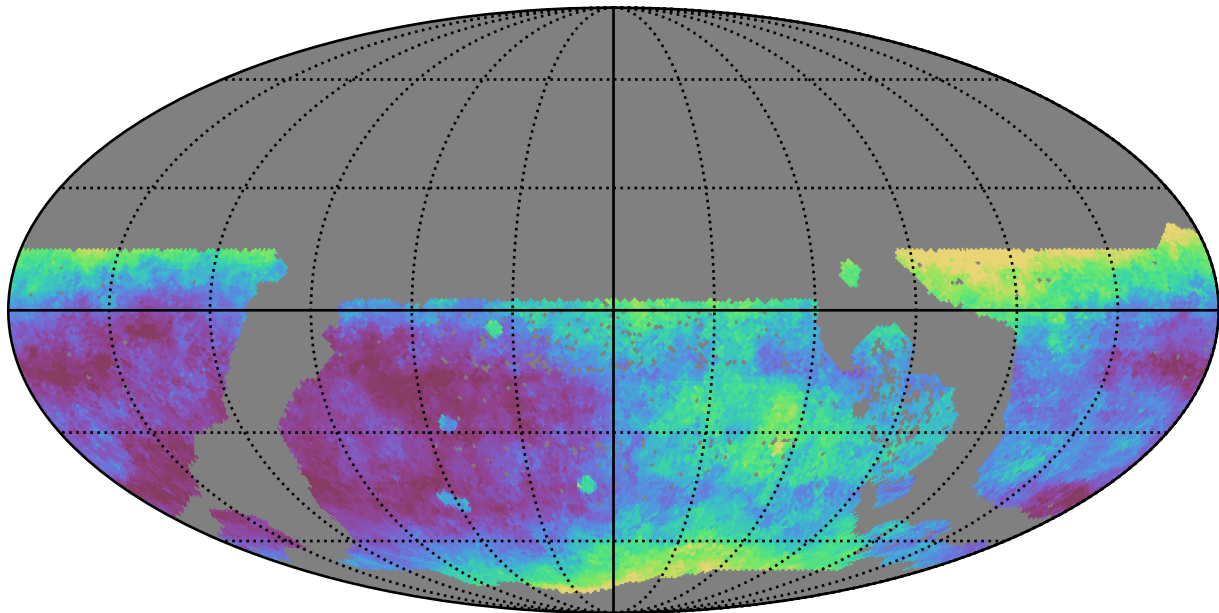
too_elab_r64_d2_gz_v3.4_10yrs WFD r band: Median seeingEff
