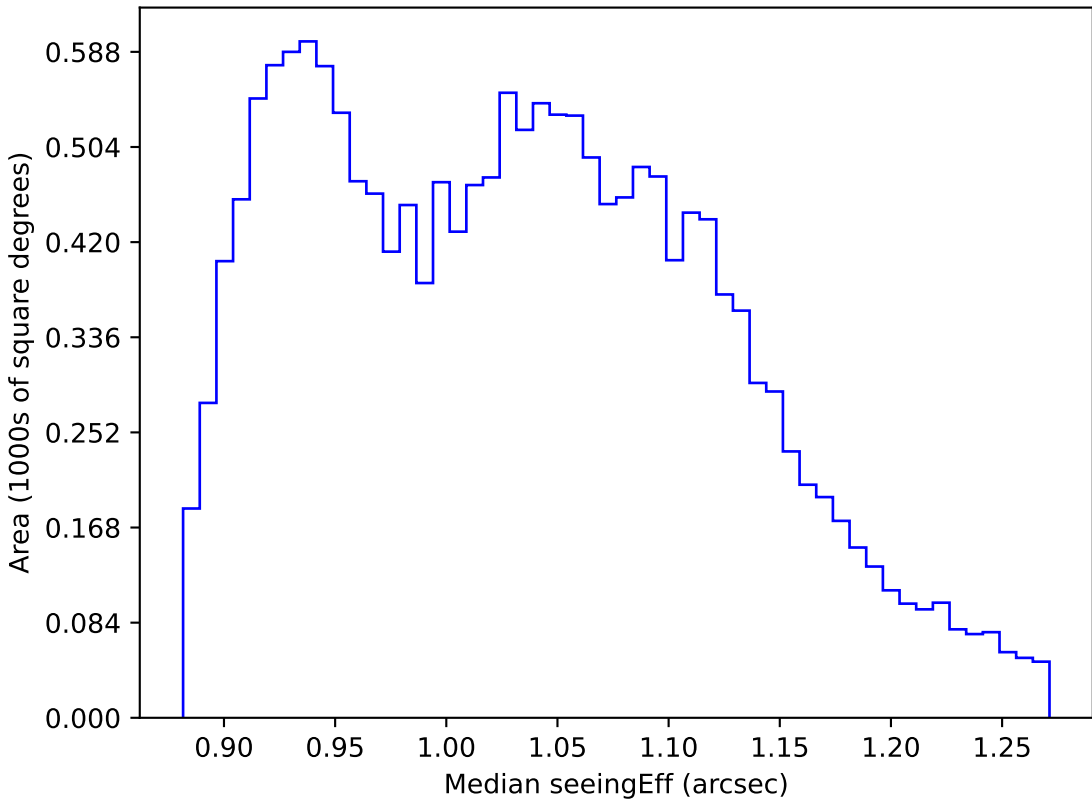
too_elab_r64_d2_gz_v3.4_10yrs WFD r band: Median seeingEff
