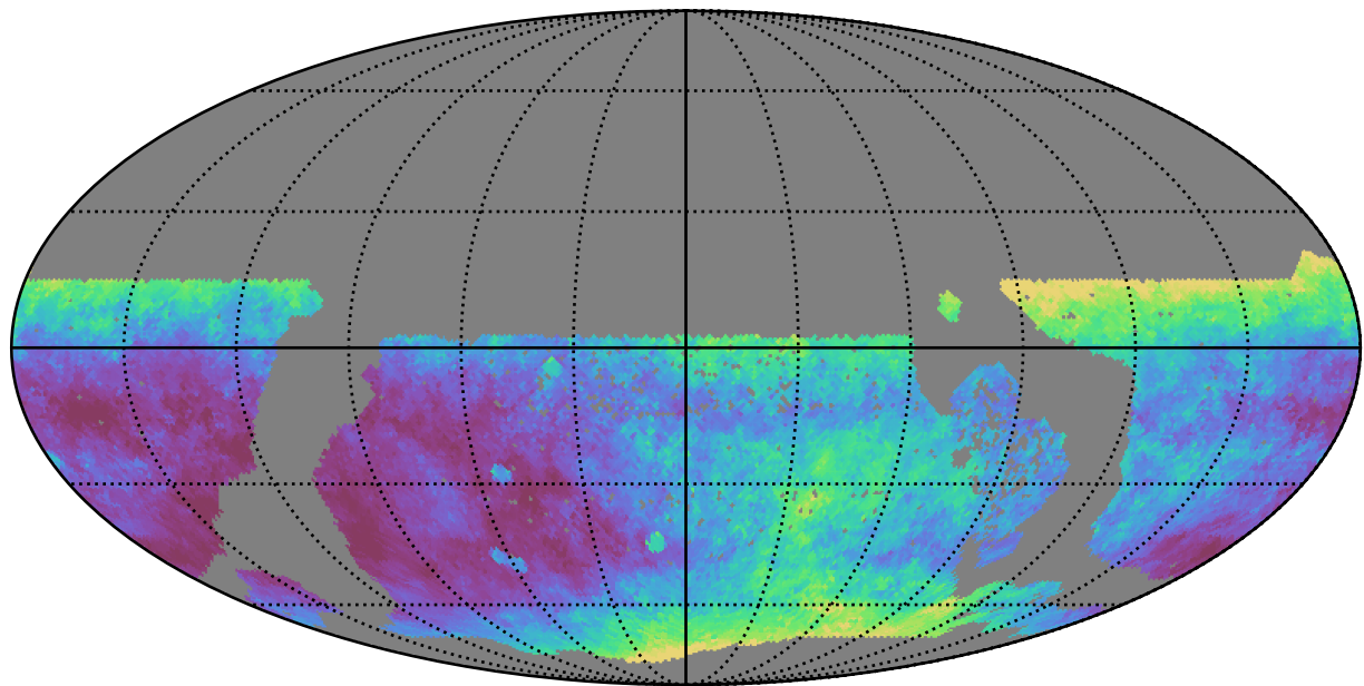
too_elab_r64_d2_gz_v3.4_10yrs WFD i band: Median seeingEff
