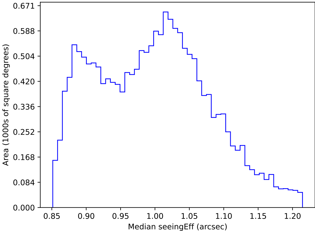
too_elab_r64_d2_gz_v3.4_10yrs WFD i band: Median seeingEff
