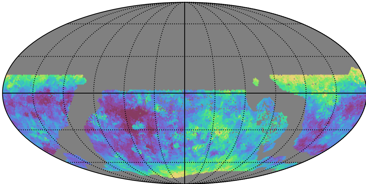
too_elab_r64_d2_gz_v3.4_10yrs WFD g band: Median seeingEff
