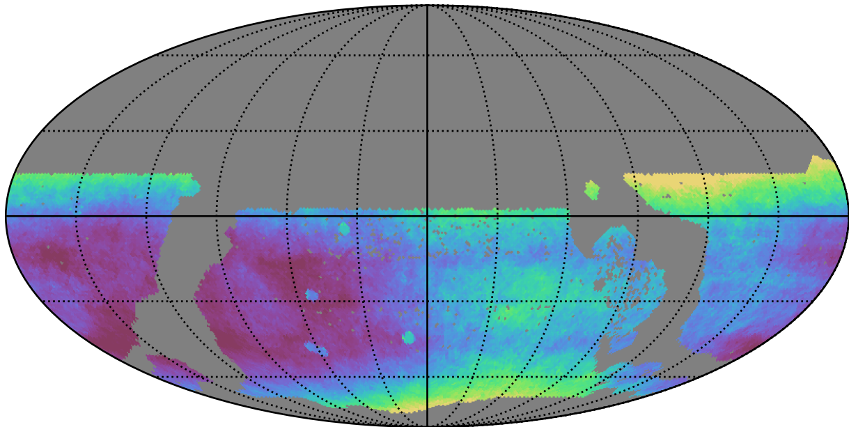
too_elab_r64_d2_gz_v3.4_10yrs WFD all bands: Median seeingEff
