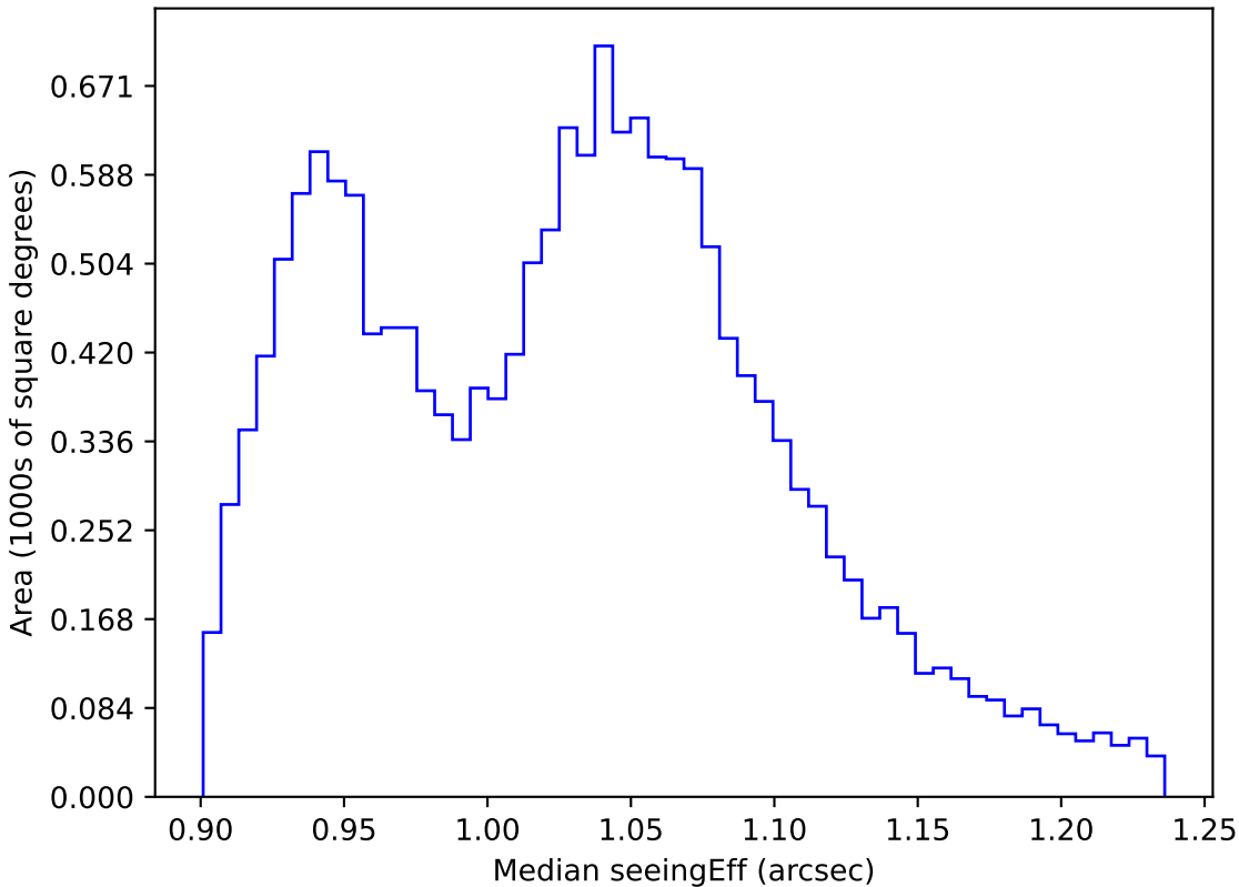
too_elab_r64_d2_gz_v3.4_10yrs WFD all bands: Median seeingEff
