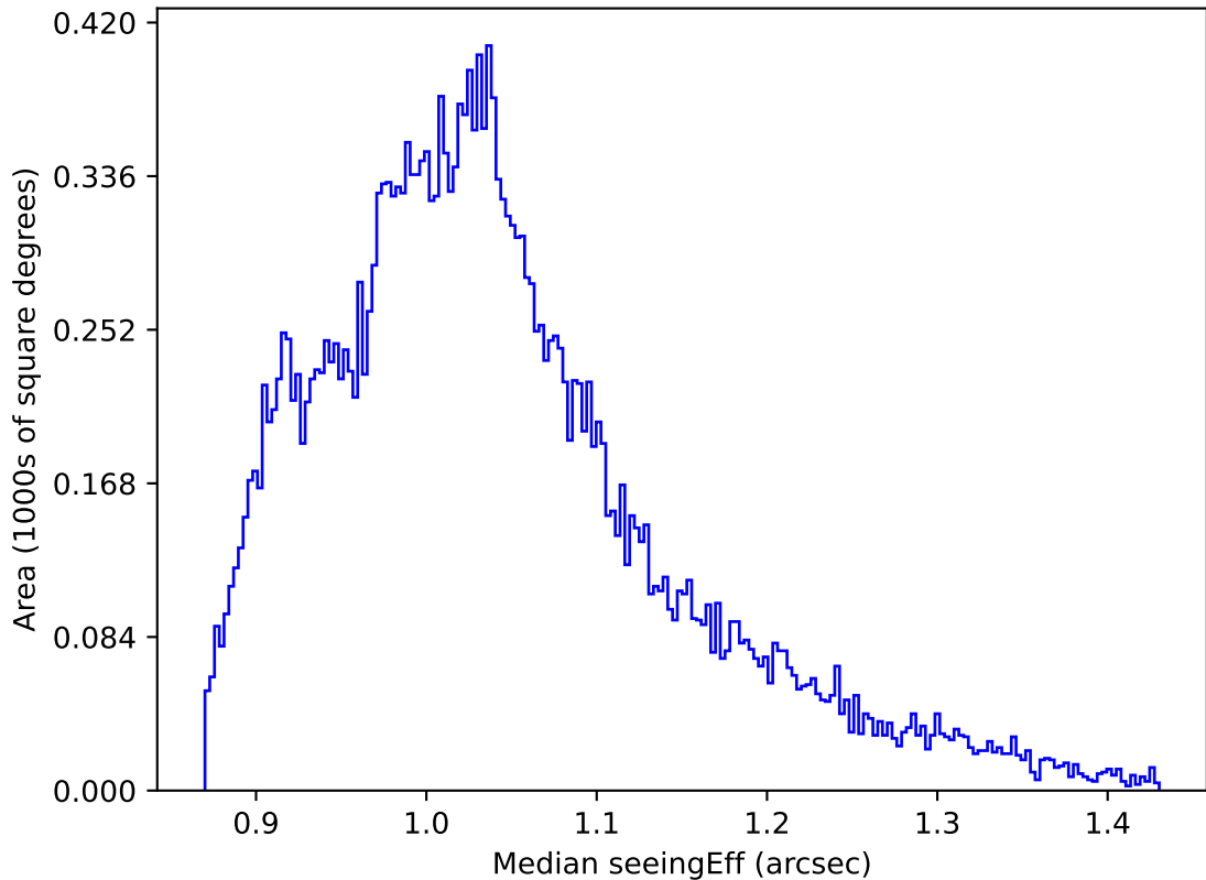
too_elab_r64_d2_gz_v3.4_10yrs All sky z band: Median seeingEff
