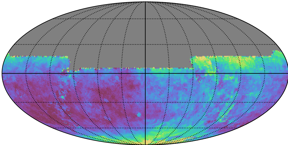
too_elab_r64_d2_gz_v3.4_10yrs All sky y band: Median seeingEff
