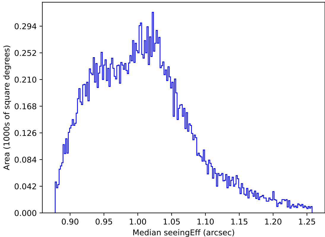
too_elab_r64_d2_gz_v3.4_10yrs All sky y band: Median seeingEff
