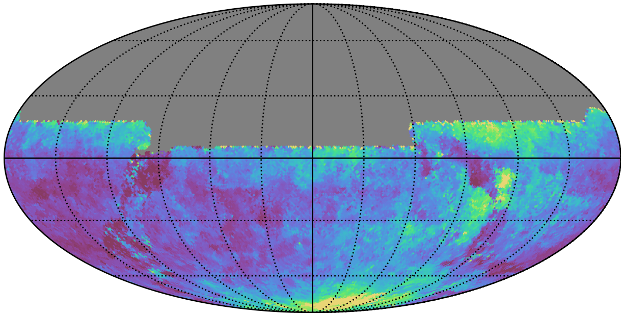
too_elab_r64_d2_gz_v3.4_10yrs All sky u band: Median seeingEff
