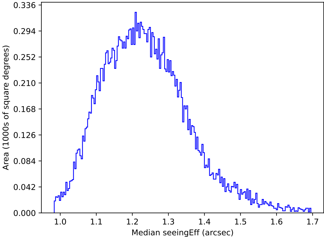
too_elab_r64_d2_gz_v3.4_10yrs All sky u band: Median seeingEff
