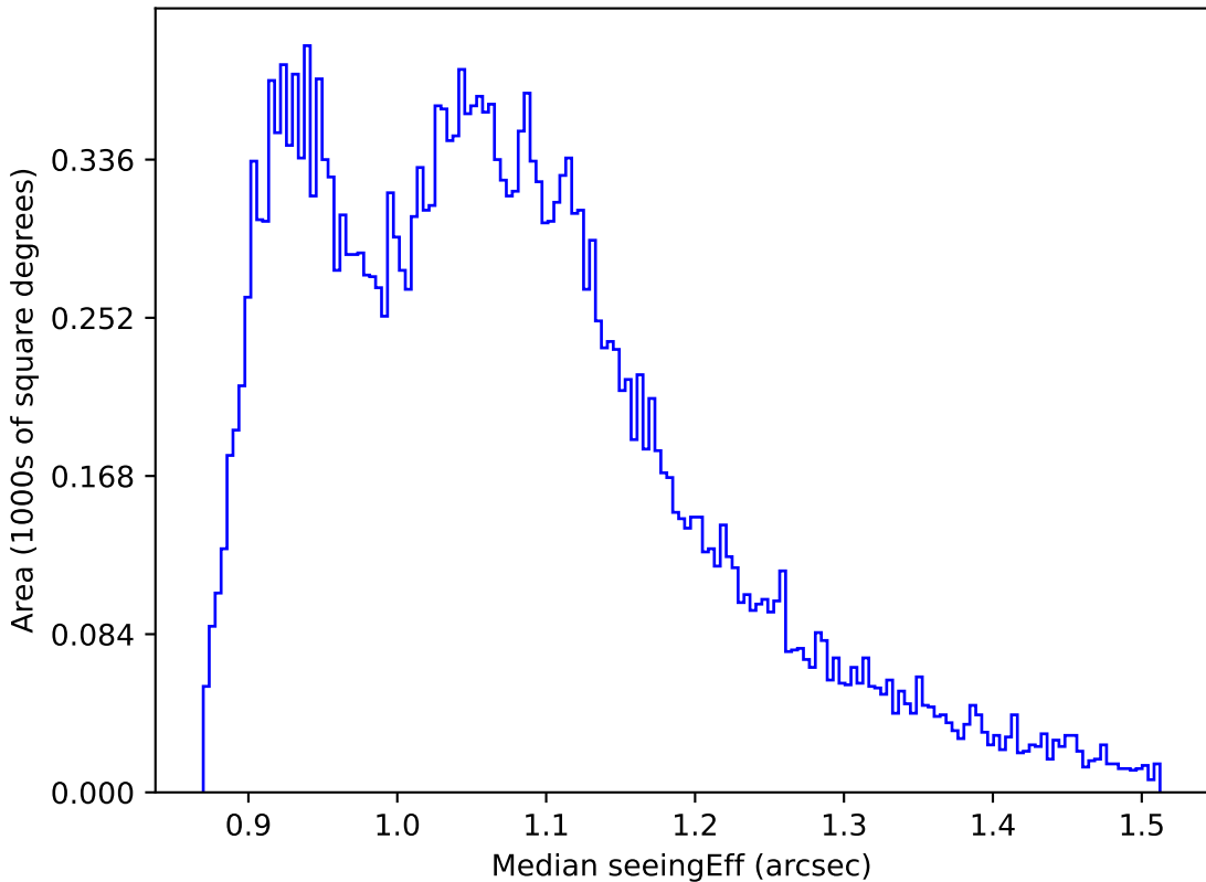
too_elab_r64_d2_gz_v3.4_10yrs All sky r band: Median seeingEff
