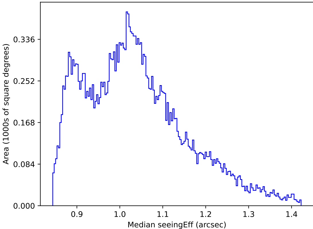
too_elab_r64_d2_gz_v3.4_10yrs All sky i band: Median seeingEff
