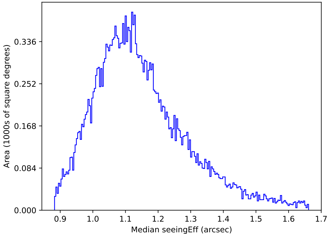
too_elab_r64_d2_gz_v3.4_10yrs All sky g band: Median seeingEff
