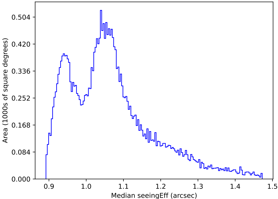
too_elab_r64_d2_gz_v3.4_10yrs All sky all bands: Median seeingEff
