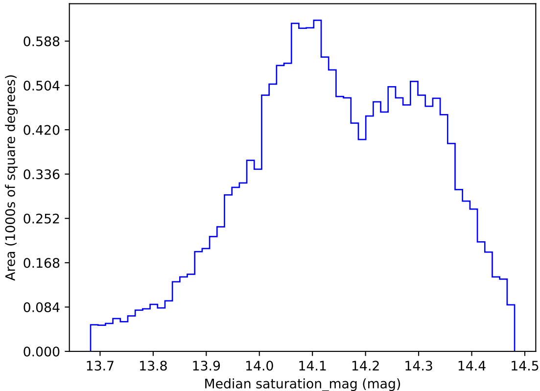
too_elab_r64_d2_gz_v3.4_10yrs WFD all bands: Median saturation_mag
