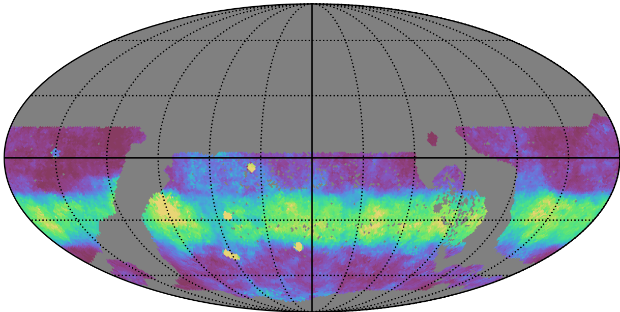
too_elab_r64_d2_gz_v3.4_10yrs WFD z band: Median normairmass
