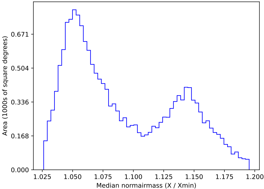
too_elab_r64_d2_gz_v3.4_10yrs WFD y band: Median normairmass
