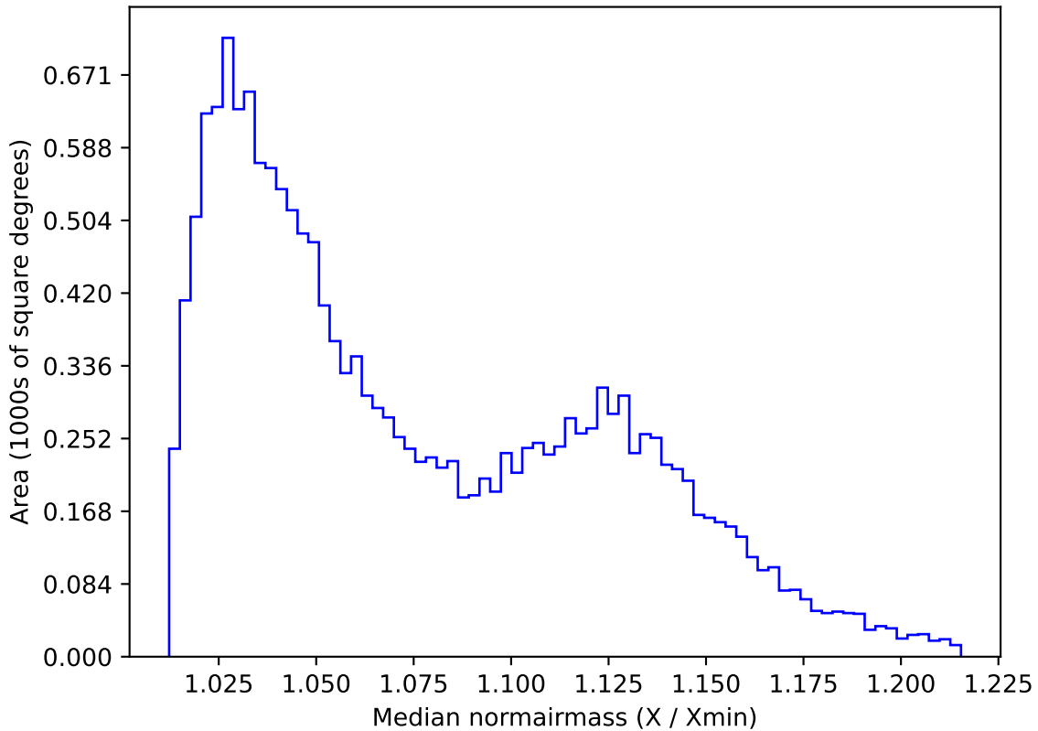
too_elab_r64_d2_gz_v3.4_10yrs WFD u band: Median normairmass
