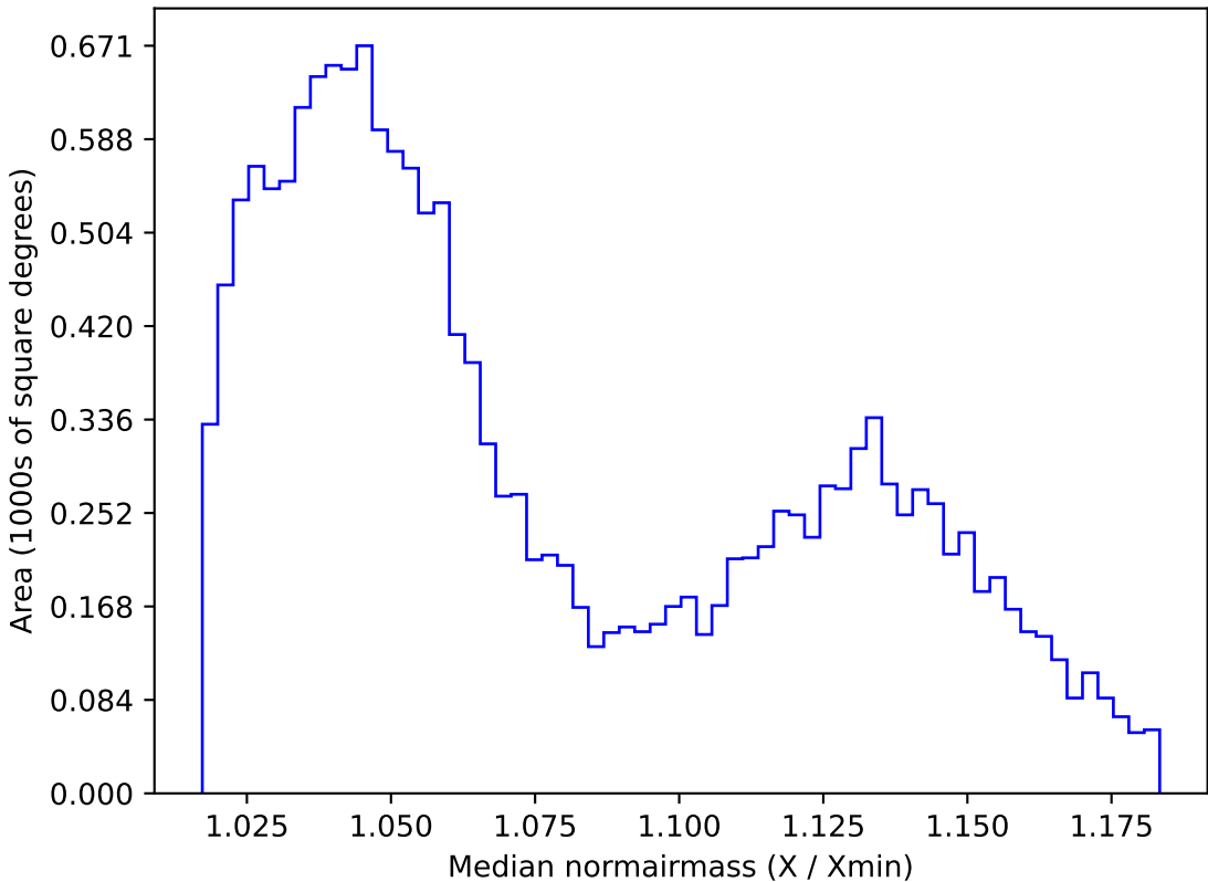
too_elab_r64_d2_gz_v3.4_10yrs WFD r band: Median normairmass
