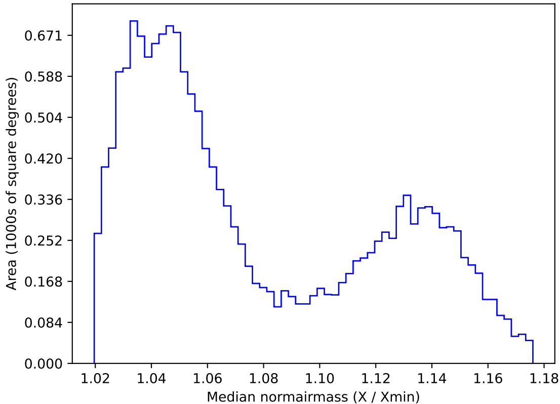
too_elab_r64_d2_gz_v3.4_10yrs WFD i band: Median normairmass
