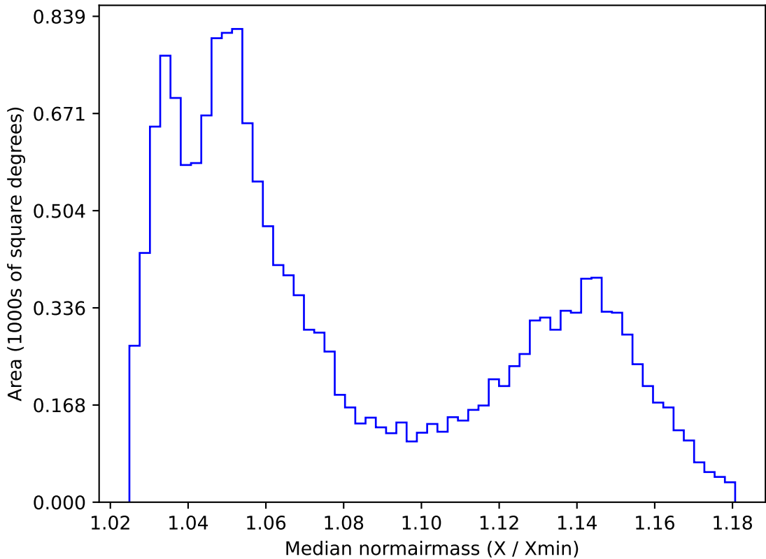
too_elab_r64_d2_gz_v3.4_10yrs WFD all bands: Median normairmass
