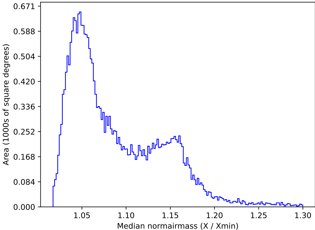
too_elab_r64_d2_gz_v3.4_10yrs All sky z band: Median normairmass
