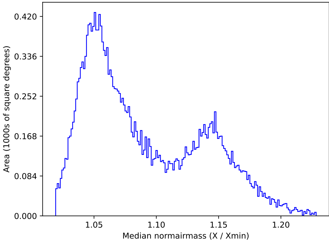
too_elab_r64_d2_gz_v3.4_10yrs All sky y band: Median normairmass
