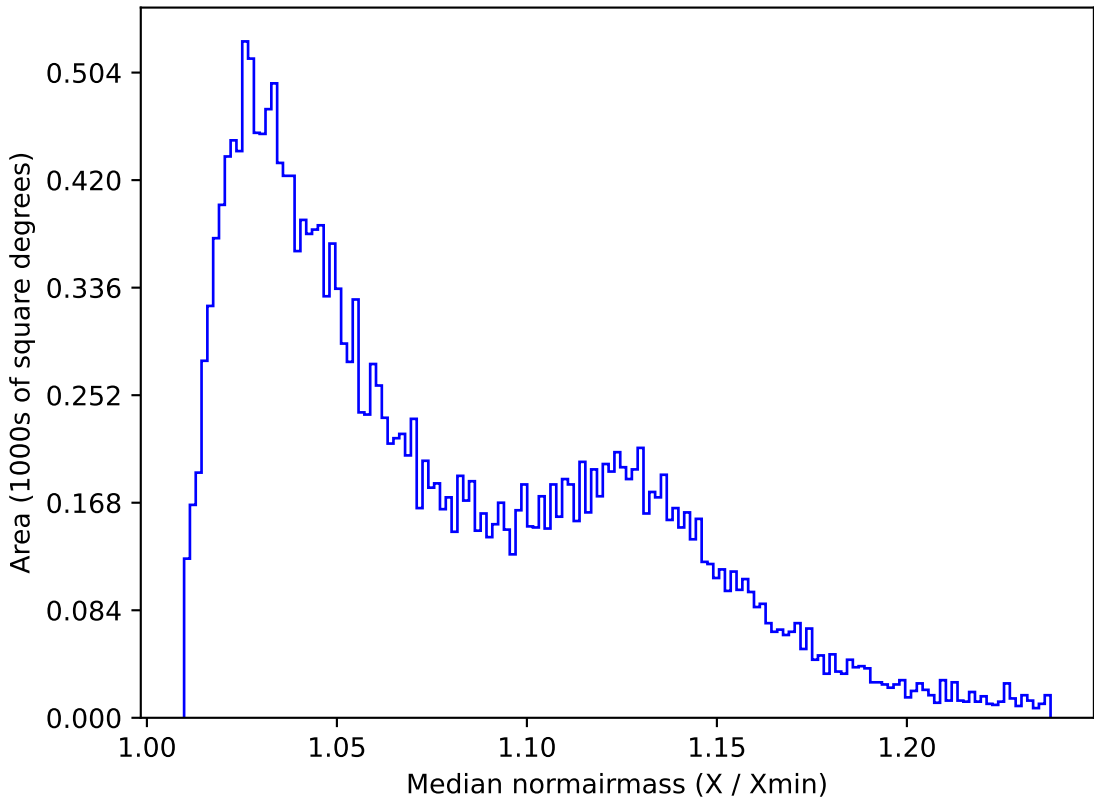
too_elab_r64_d2_gz_v3.4_10yrs All sky u band: Median normairmass
