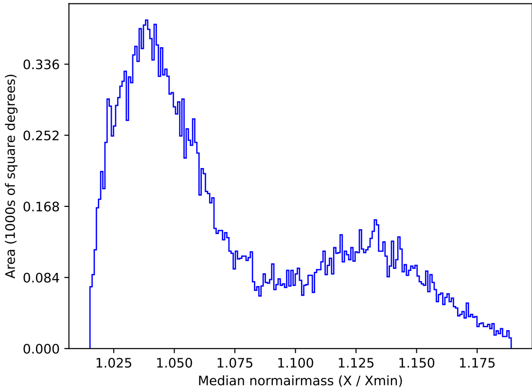
too_elab_r64_d2_gz_v3.4_10yrs All sky r band: Median normairmass
