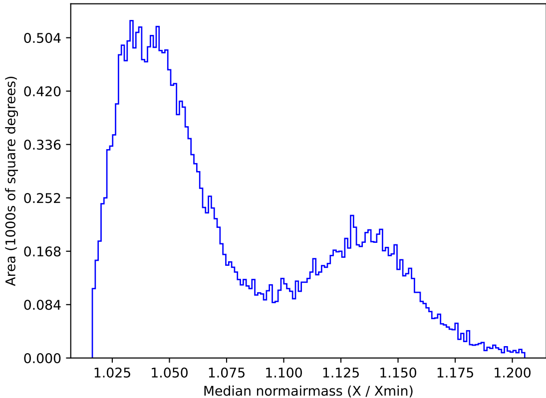
too_elab_r64_d2_gz_v3.4_10yrs All sky i band: Median normairmass
