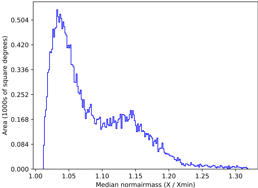
too_elab_r64_d2_gz_v3.4_10yrs All sky g band: Median normairmass
