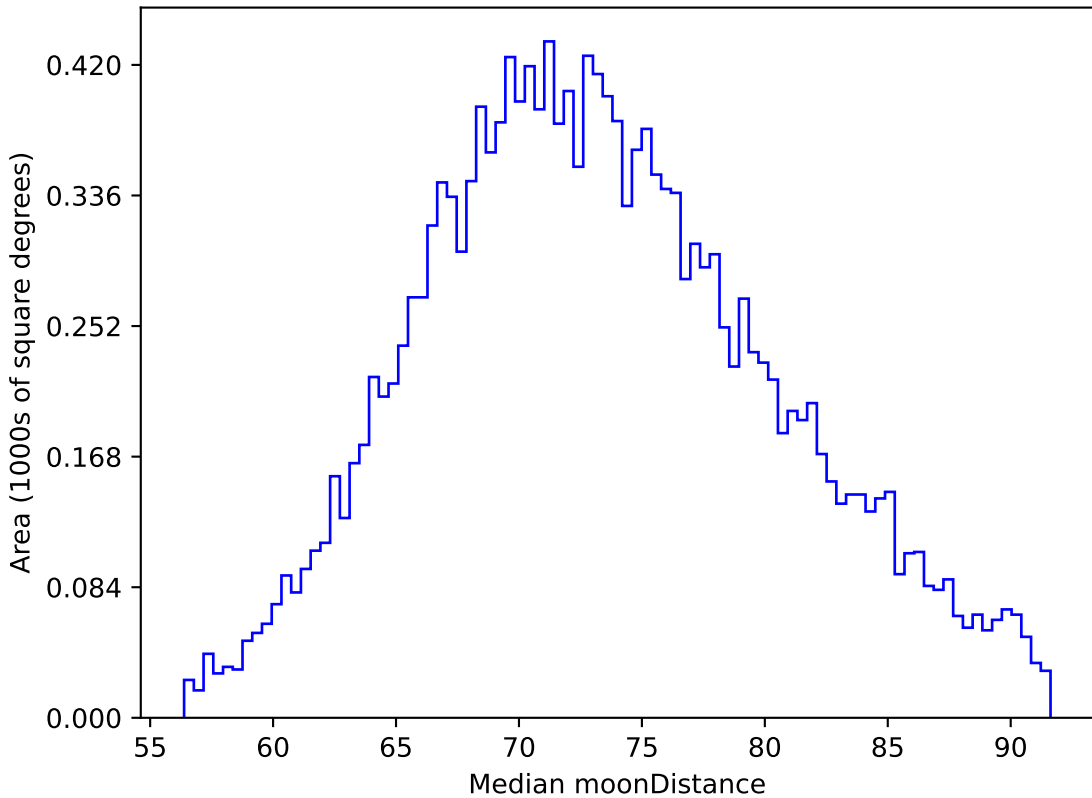
too_elab_r64_d2_gz_v3.4_10yrs WFD z band: Median moonDistance
