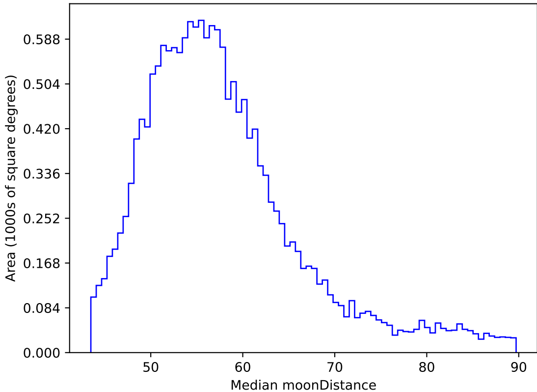
too_elab_r64_d2_gz_v3.4_10yrs WFD y band: Median moonDistance
