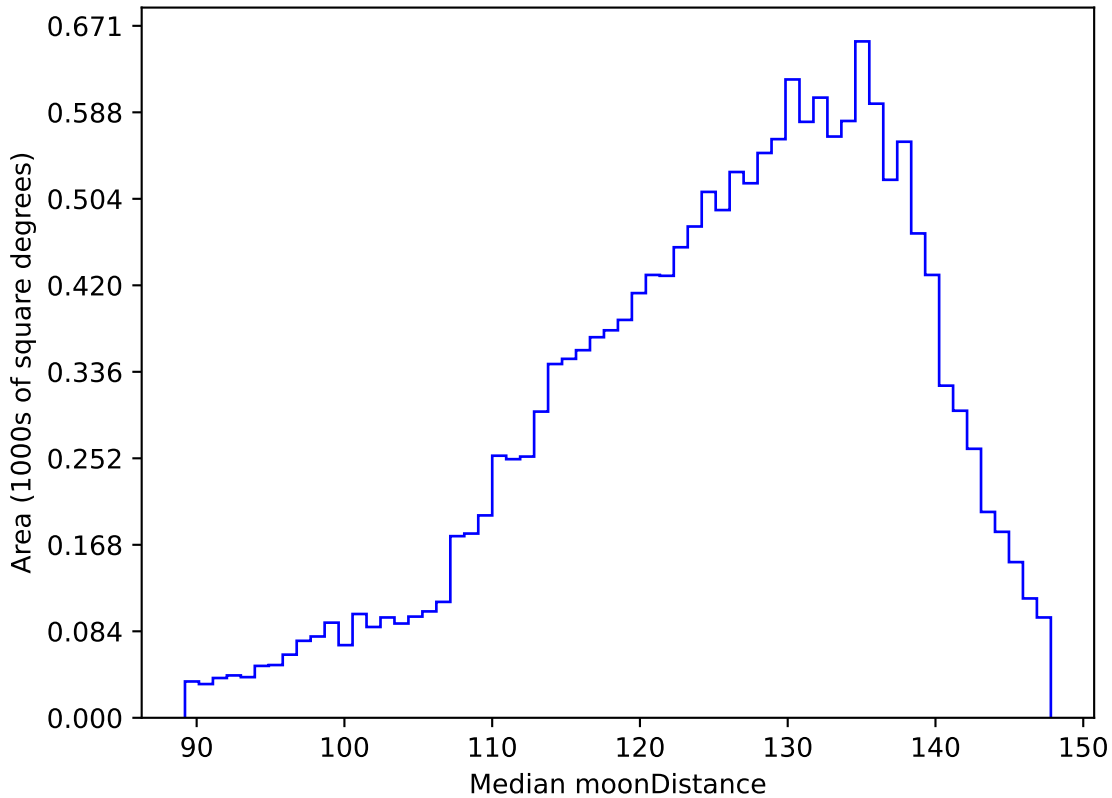
too_elab_r64_d2_gz_v3.4_10yrs WFD u band: Median moonDistance
