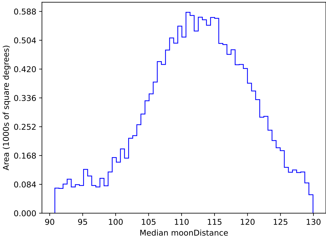
too_elab_r64_d2_gz_v3.4_10yrs WFD r band: Median moonDistance
