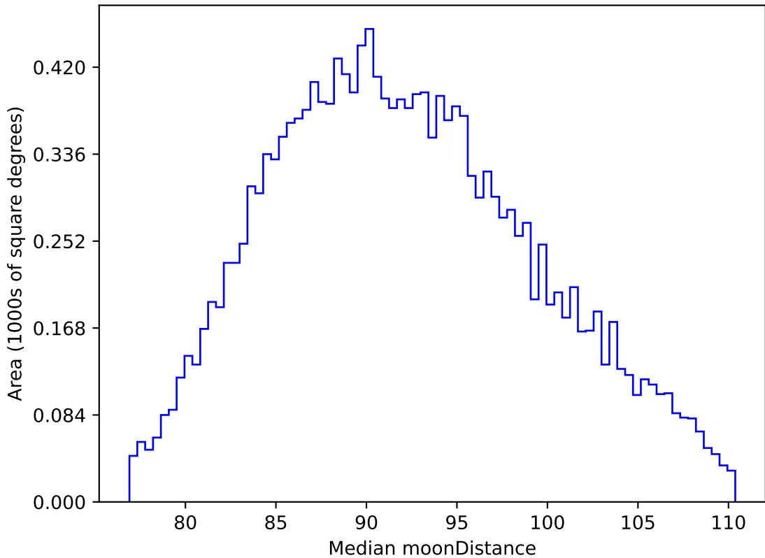
too_elab_r64_d2_gz_v3.4_10yrs WFD i band: Median moonDistance
