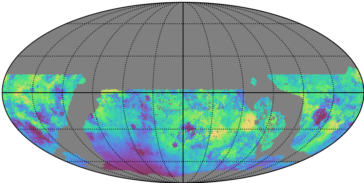
too_elab_r64_d2_gz_v3.4_10yrs WFD g band: Median moonDistance
