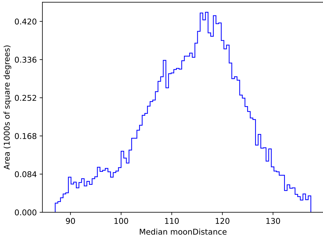
too_elab_r64_d2_gz_v3.4_10yrs WFD g band: Median moonDistance
