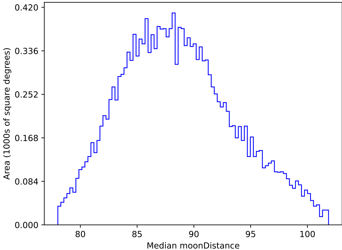
too_elab_r64_d2_gz_v3.4_10yrs WFD all bands: Median moonDistance
