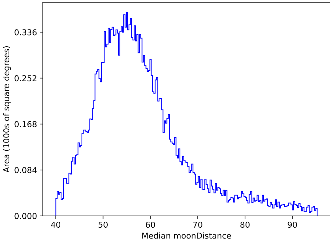
too_elab_r64_d2_gz_v3.4_10yrs All sky y band: Median moonDistance
