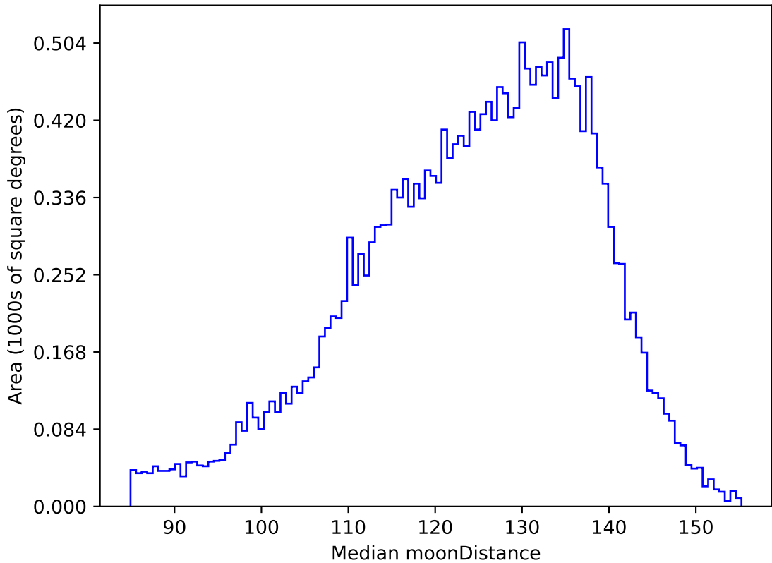
too_elab_r64_d2_gz_v3.4_10yrs All sky u band: Median moonDistance
