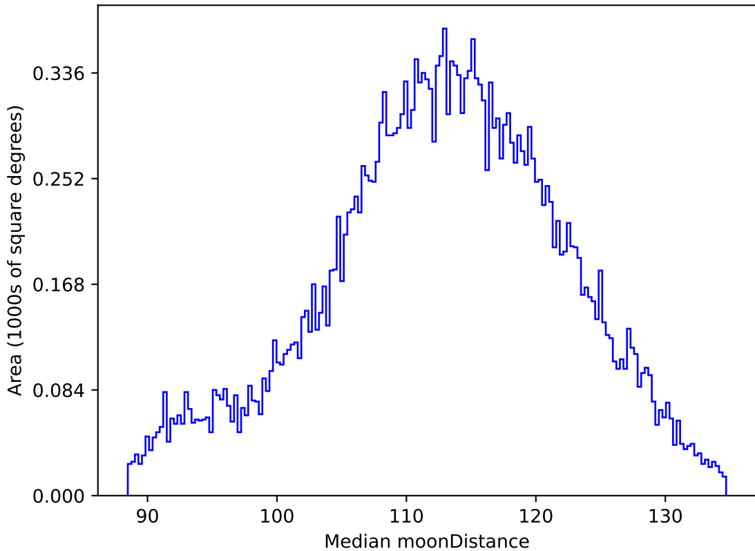
too_elab_r64_d2_gz_v3.4_10yrs All sky r band: Median moonDistance
