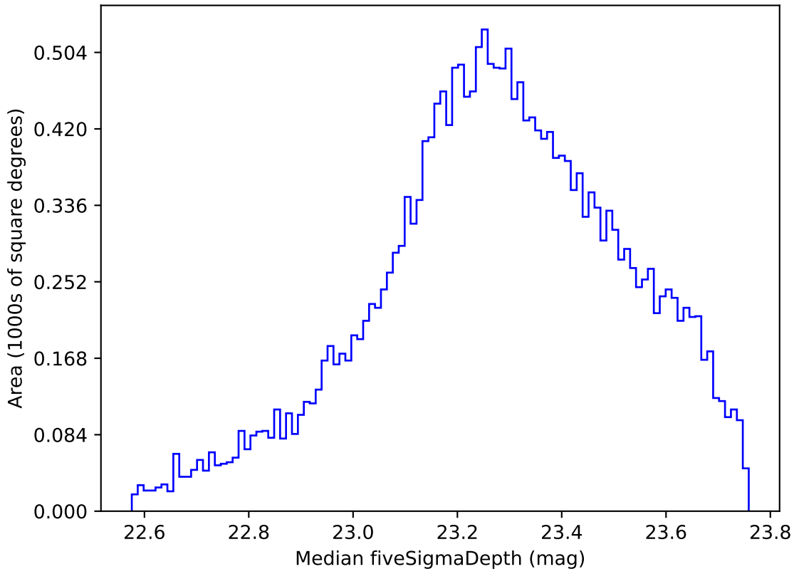
too_elab_r64_d2_gz_v3.4_10yrs Yr 1 u band: Median fiveSigmaDepth
