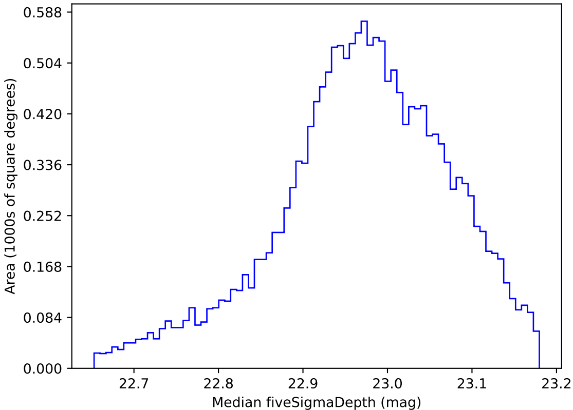
too_elab_r64_d2_gz_v3.4_10yrs WFD z band: Median fiveSigmaDepth
