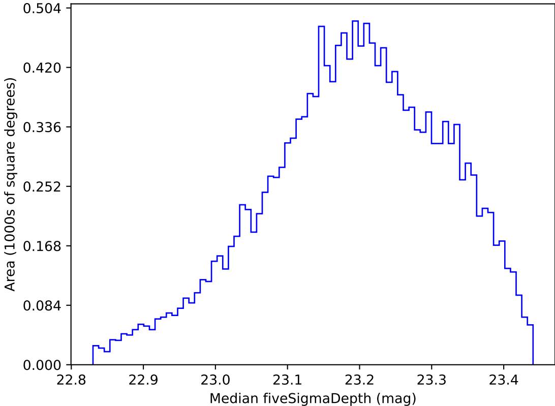
too_elab_r64_d2_gz_v3.4_10yrs WFD u band: Median fiveSigmaDepth
