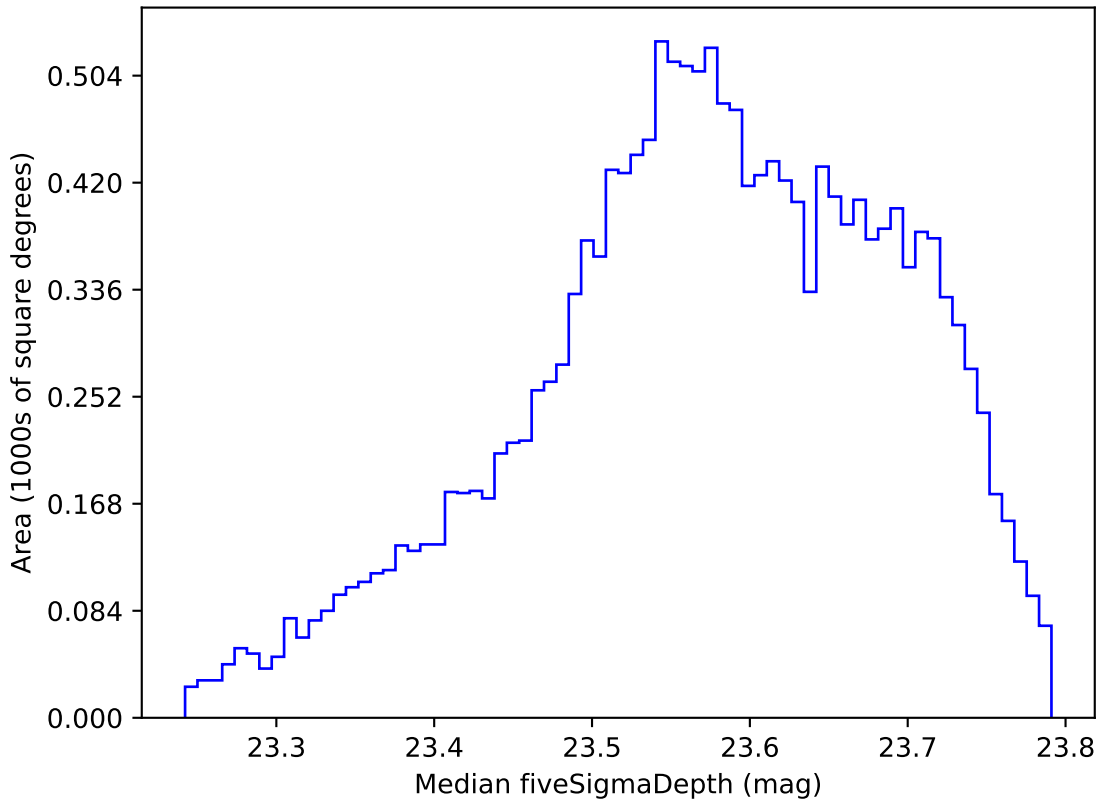
too_elab_r64_d2_gz_v3.4_10yrs WFD i band: Median fiveSigmaDepth
