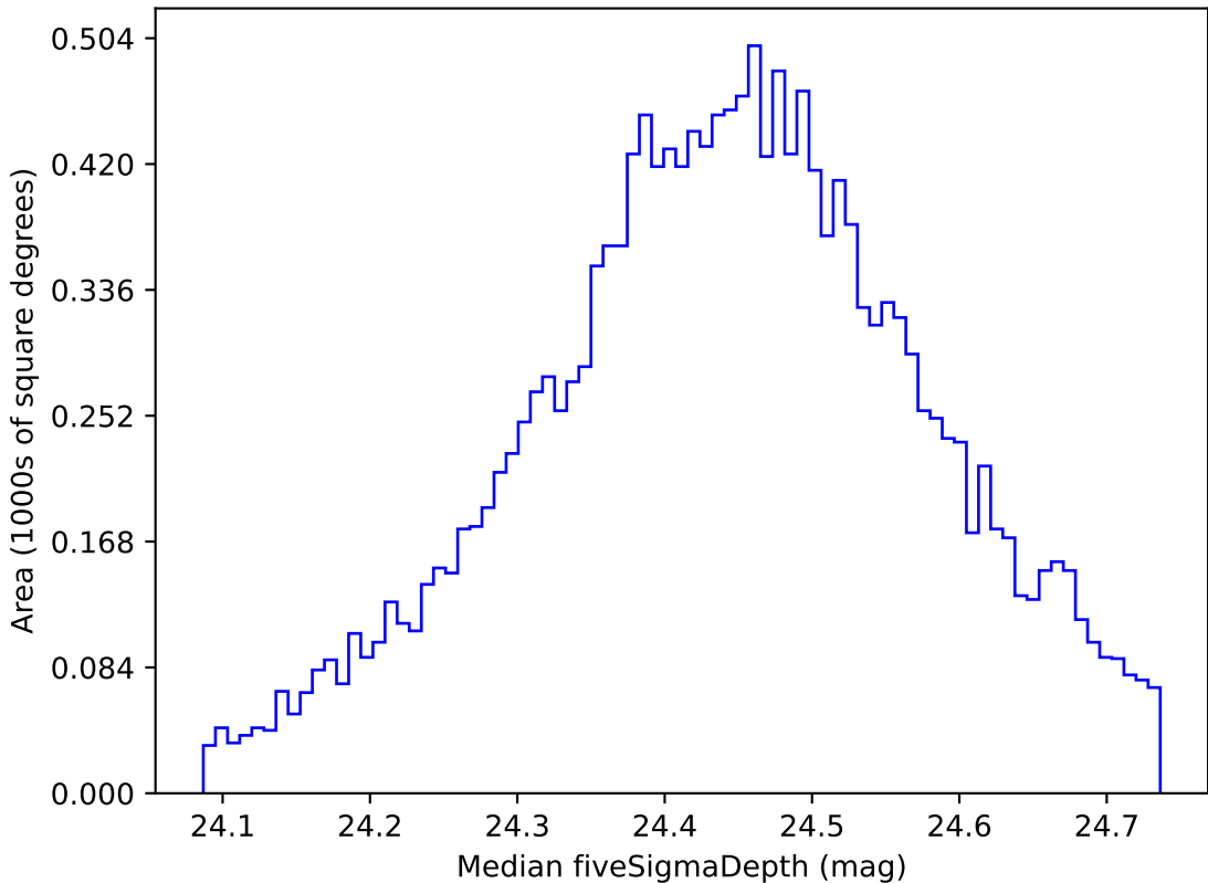
too_elab_r64_d2_gz_v3.4_10yrs WFD g band: Median fiveSigmaDepth
